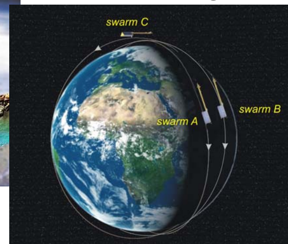
SWARM
